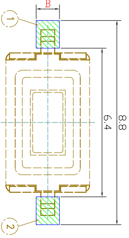
P.C.B MOUNTING PATTERN DIMENSION The following soldering are recommended for reflow soldering
